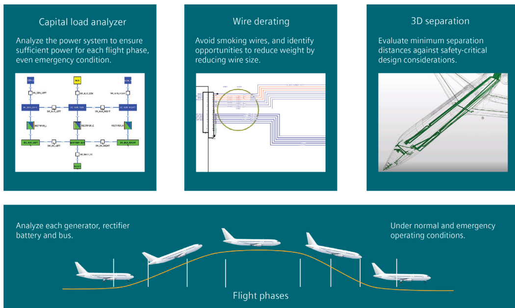
Figure 4. The Capital compliance solution ensures safe electrical design in all flight operations.
