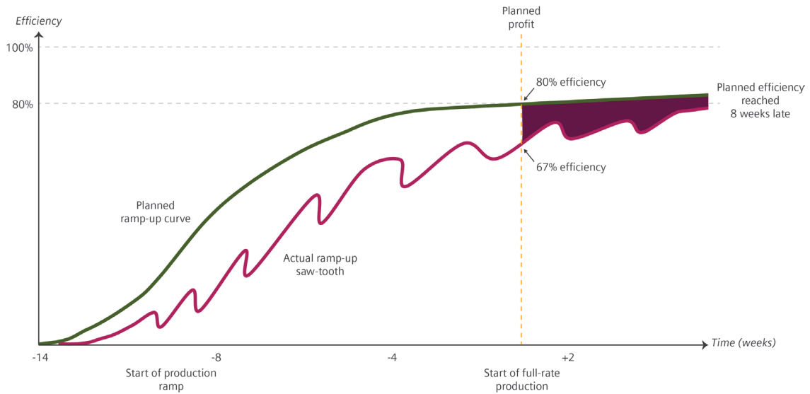
Figure 5. Traditional “planned” production ramp versus typical “actual” ramp.
